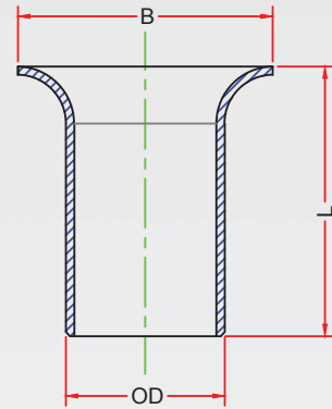
SECTIONAL VIEW
